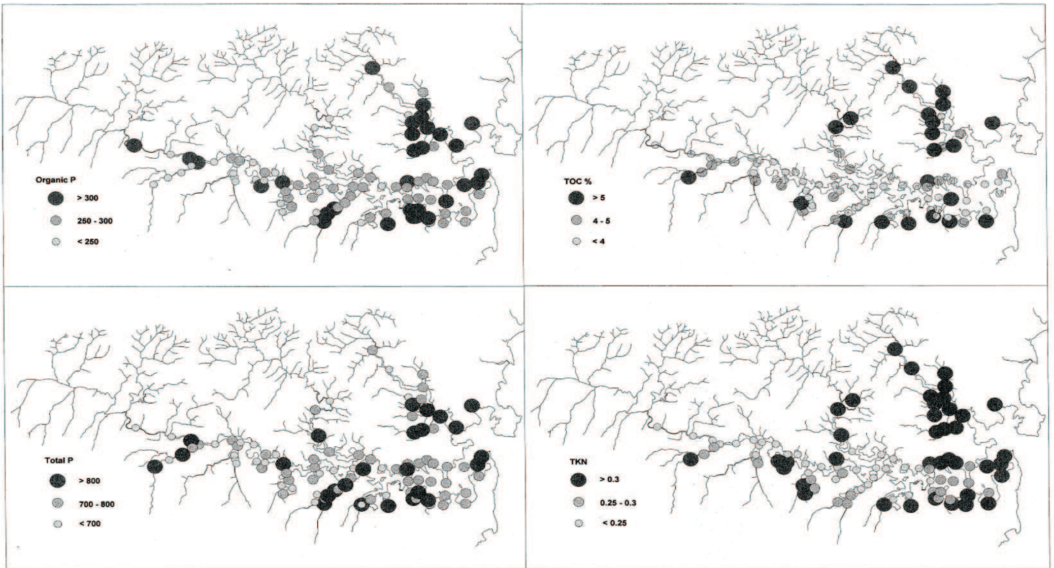
The distribution of Organic Phosphorus (P), Total Organic Carbon (TOC), Total Phosphorus and Total Kjeldahl Nitrogen (TKN) in fine fraction (<63µm) of surficial sediment.
